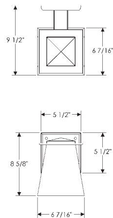
LANTERN SCONCE WS465 Weight: 27 lbs. Shown with the E403 5 1/2" square escutcheon in silicon bronze, dark patina. UL rated for wet location.
