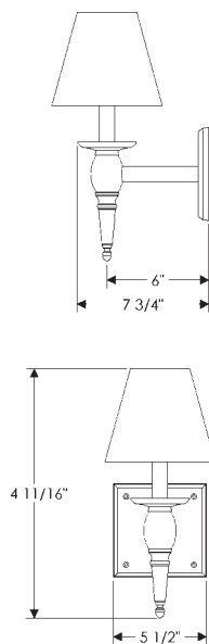
TOWNE SCONCE WS500 Weight: 6 1/2 lbs. Shown with the E403 5 1/2" square escutcheon in silicon bronze, light patina. Fabric shade options, crystals, and prism are available as shown. See rockymountainhardware.com.
