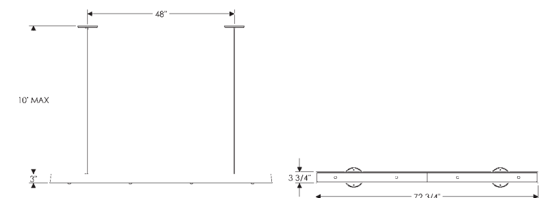
LINEAR CHANDELIER C420 Weight: 65 lbs. Shown in silicon bronze, light patina. Maximum standard length is 10".
