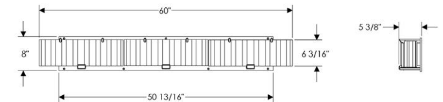
TRIPLE PLANK SCONCE—CORRUGATED GLASS V445 Weight: 60 lbs. Shown in white bronze, dark patina.
